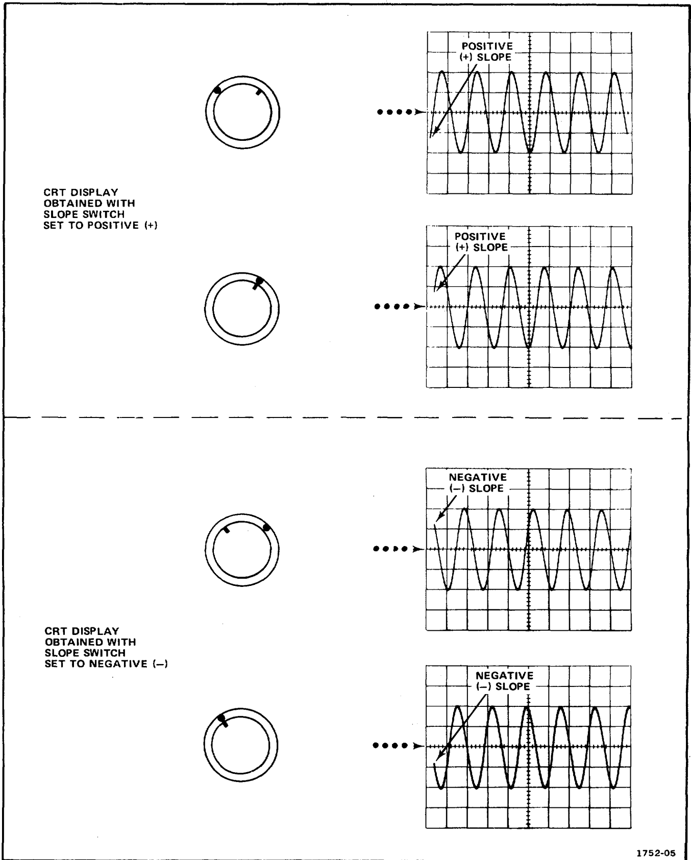
Figure 2-4. Effect of LEVEL control and SLOPE switch on CRT display.
